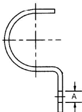
FIG. 233 ONE HOLE PIPE STRAP
