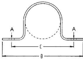
FIG. 231SS TWO HOLE PIPE STRAP, 304 STAINLESS STEEL, IPS FIG. 231OD TWO HOLE PIPE STRAP, 304 STAINLESS STEEL, O.D.
