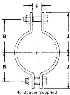
FIG. 216 HEAVY DUTY TWO-BOLT PIPE CLAMP
