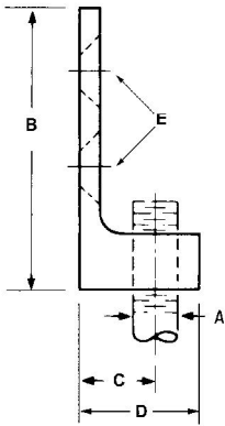
FIG. 153 SIDE BEAM CONNECTOR
