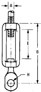
FIG. 114 TURNBUCKLE ADJUSTER
